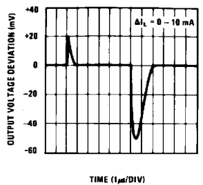
Load Transient Response for Positive Regulator
