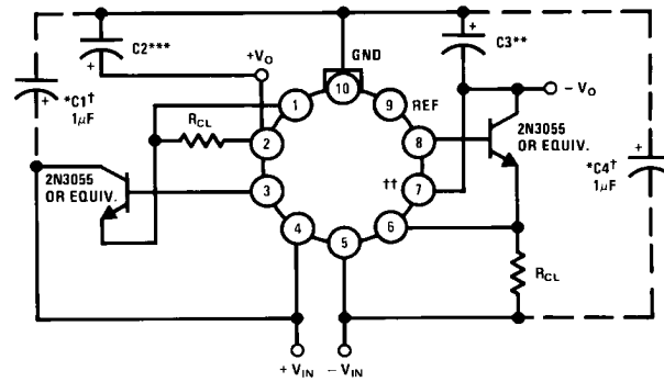
2.0 Amp Boosted Regulator with Current Limit
