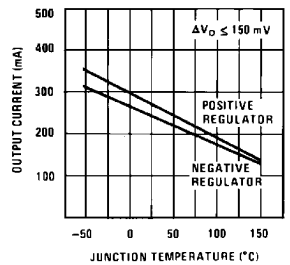
Peak Output Current vs Junction Temperature
