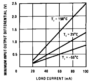
Regulator Dropout Voltage for Negative Regulator
