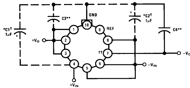
Basic Regulator†††
