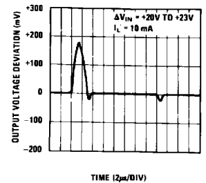
Line Transient Response for Positive Regulator
