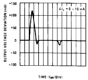
Load Transient Response for Negative Regulator
