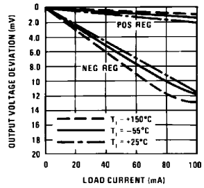
Load Regulation
