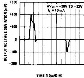
Line Transient Response for Negative Regulator
