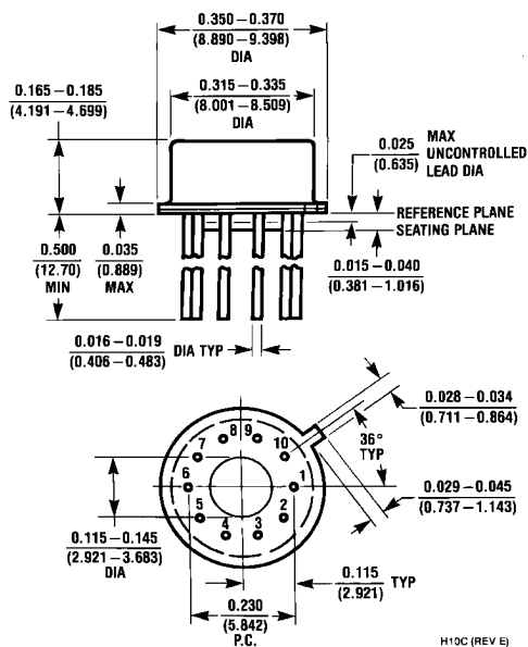
Metal Can Package (H) Order Number LM325H NS Package Number H10C
