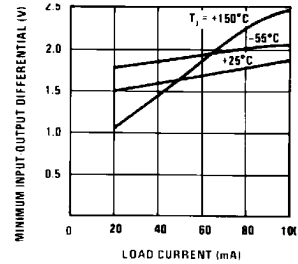
Regulator Dropout Voltage for Positive Regulator
