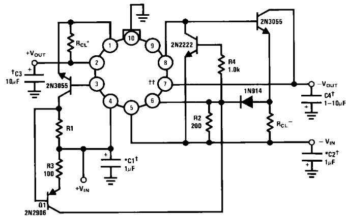
Positive Current Dependent Simultaneous Current Limiting
