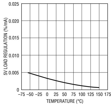
5V Load Regulation vs Temperature
