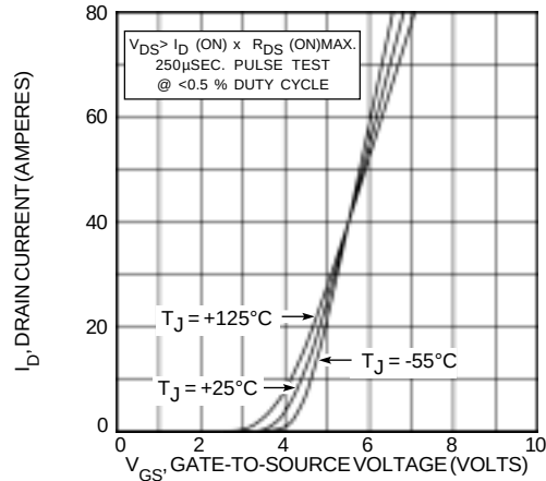
FIGURE 4, TRANSFER CHARACTERISTICS
