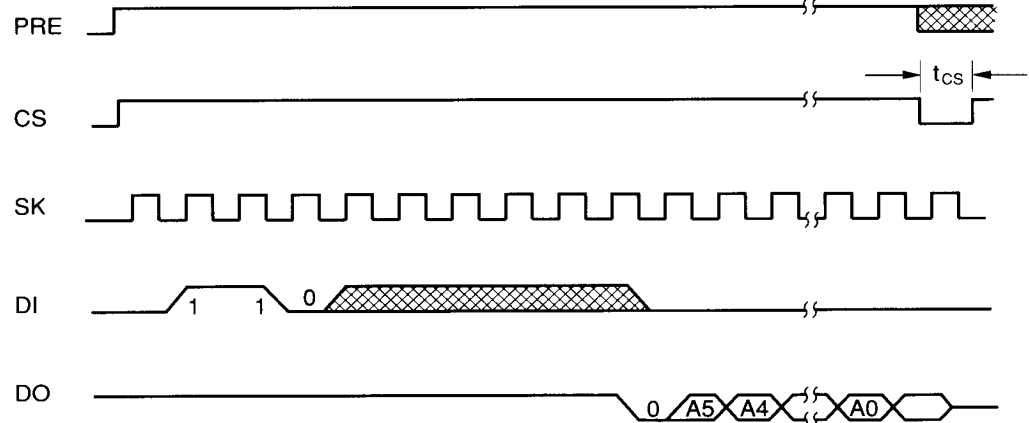
FIGURE 8. PROTECT REGISTER READ (PRREAD) CYCLE TIMING
