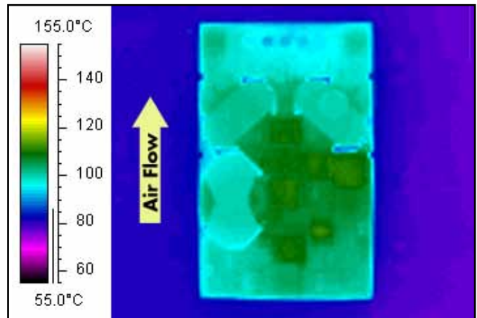
Figure 10: Thermal plot of converter at 9 amp load current with 85°C air flowing at the rate of 200 LFM. Air is flowing across the converter from input to output (24V input).
