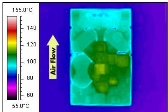
Figure 12: Thermal plot of converter at 8.7 amp load current with 85°C air flowing at the rate of 200 LFM. Air is flowing across the converter from input to output (48V input).
