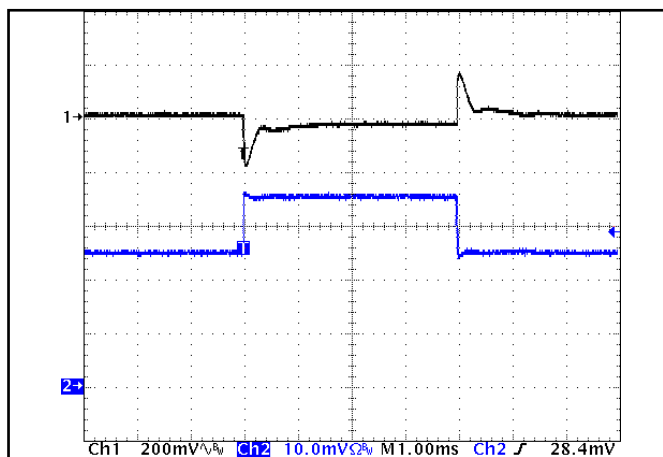
Figure 16: Output voltage response to step-change in load current (50%-75%-50% of Iout(max); di/dt = 5A/\mu s ). Load cap: 470 \mu F , 30 m \Omega ESR tantalum cap and 1 \mu F ceramic cap. Ch 1: Vout (200mV/div), Ch 2: Iout (2A/div).
