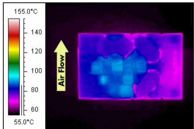
Figure 6: Thermal plot of converter at 9 amp load current with 55°C air flowing at the rate of 200 LFM. Air is flowing across the converter sideways from pin 3 to pin 1 (24V input).
