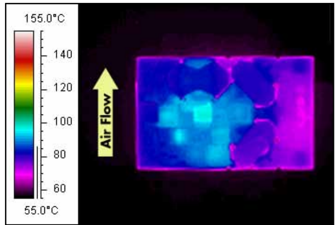
Figure 8: Thermal plot of converter at 9 amp load current with 55°C air flowing at the rate of 200 LFM. Air is flowing across the converter sideways from pin 3 to pin 1 (48V input).
