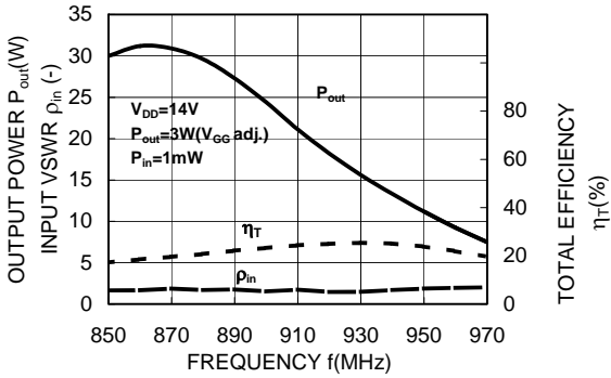
OUTPUT POWER, TOTAL EFFICIENCY, and INPUT VSWR versus FREQUENCY
