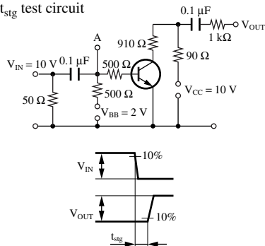
t_{sig} test circuit
