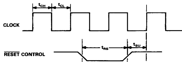
Figure 2. ADSP-3211 Reset Timing
