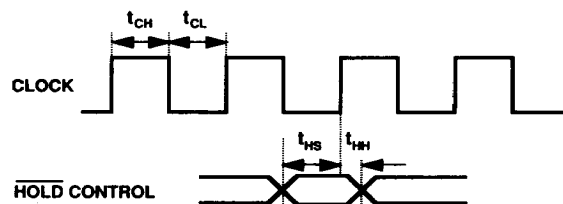
Figure 3. ADSP-3211 Multiplier Output Register Hold Timing
