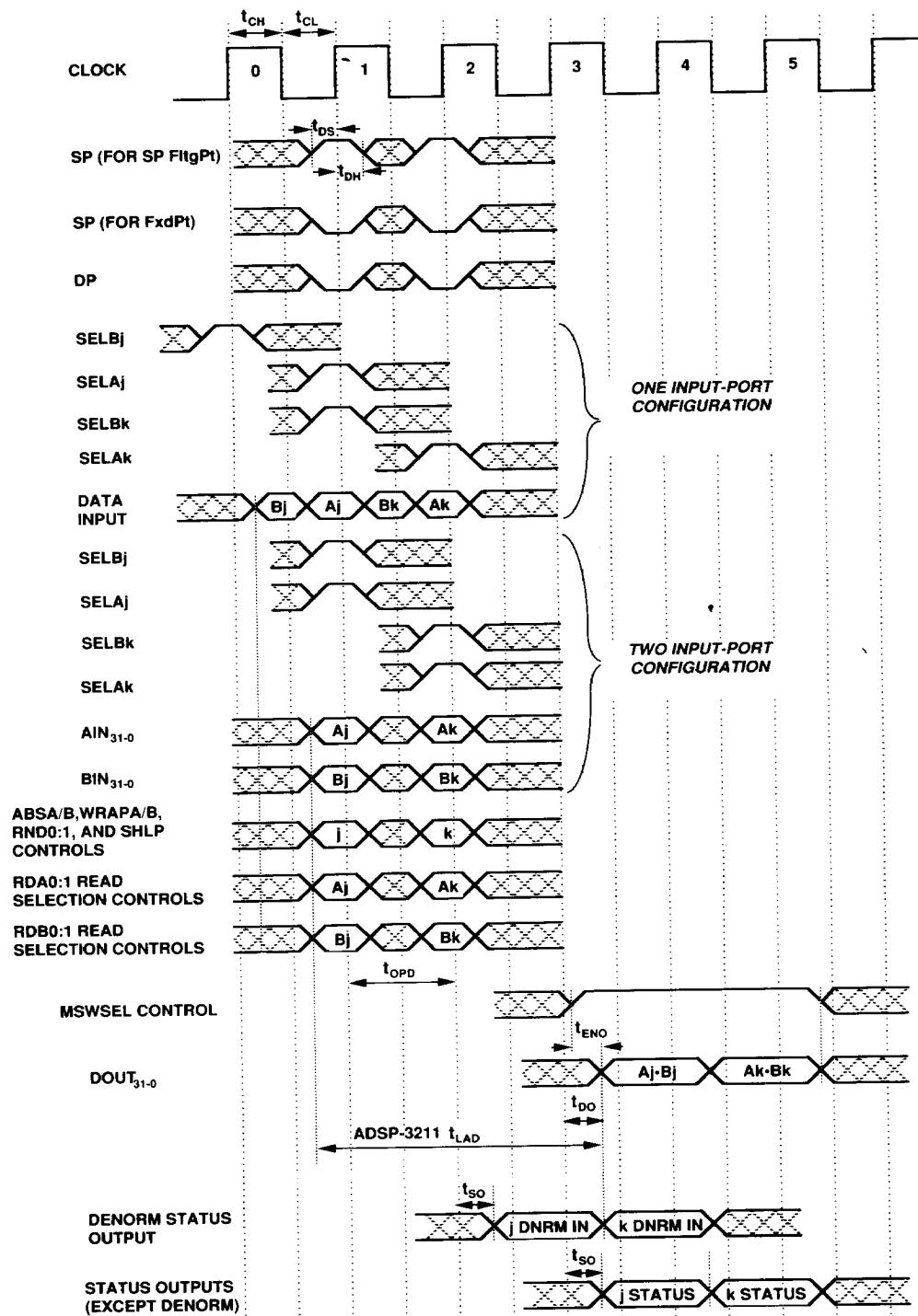
Figure 4. ADSP-3211 32-Bit Single-Precision Floating-Point and Fixed-Point Multiplications
