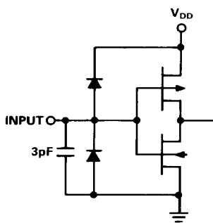
Figure 10. Equivalent Input Circuits
