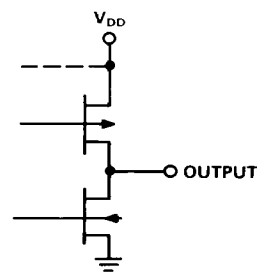
Figure 11. Equivalent Output Circuits
