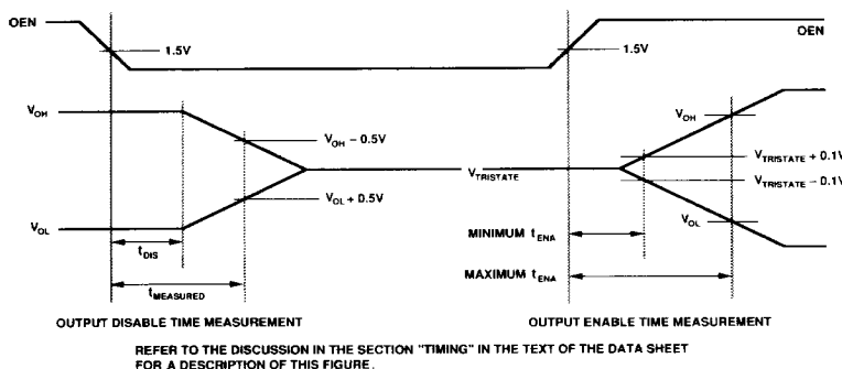
Figure 1. Three-State Disable and Enable Timing
