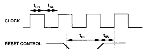
Figure 2. Reset Timing
