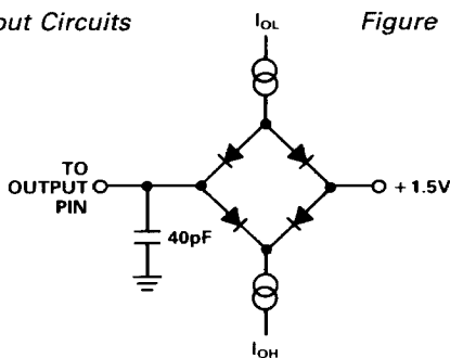
Figure 12. Normal Load for AC Measurements
