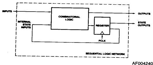
Figure 1. Sequential Network
