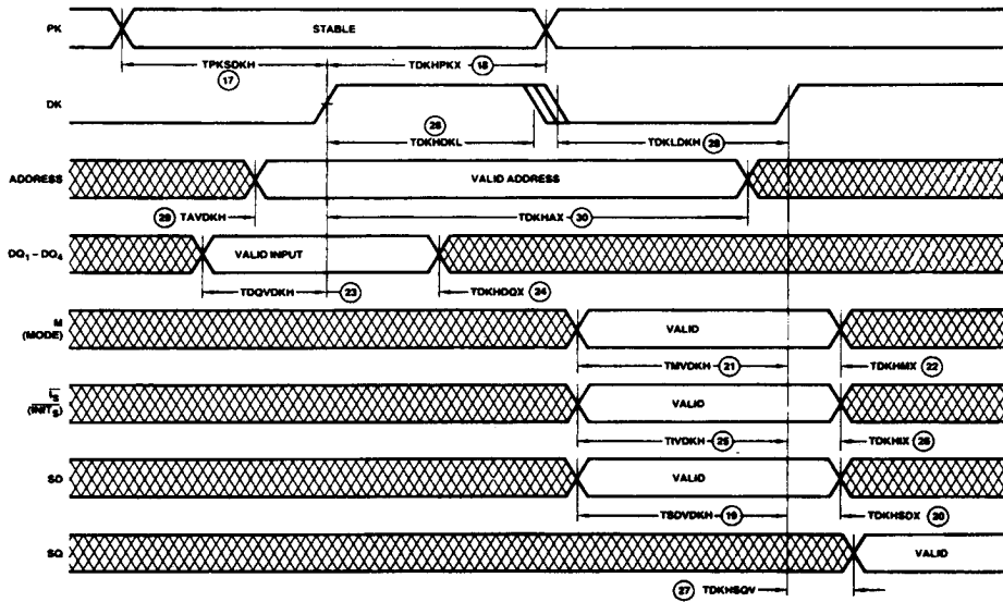
TIMING SET 3
