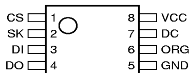
8-Pin TSSOP
