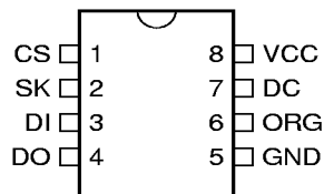
8-Pin PDIP
