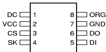
8-Pin SOIC Rotated (R) (1K JEDEC Only)
