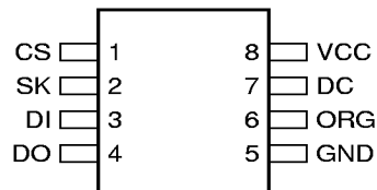
8-Pin SOIC
