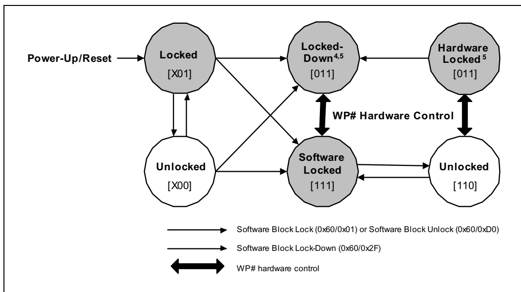
Figure 10. Block Locking State Diagram
