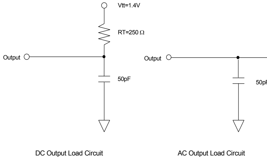
DC Output Load Circuit
