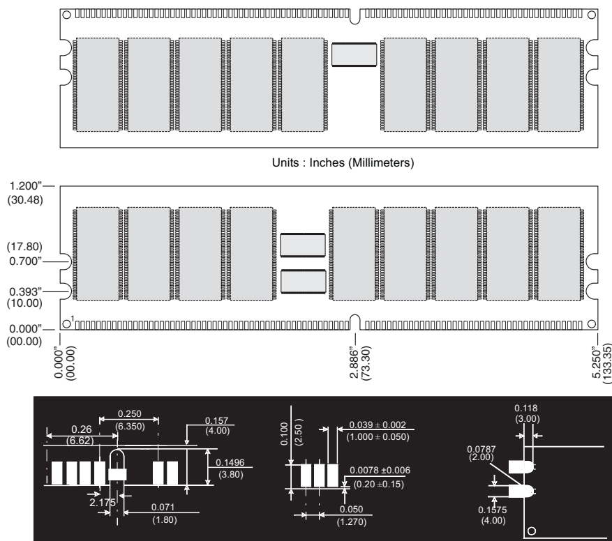
Figure 1: KVR333X72RC25/1GD 184-Pin DIMM
