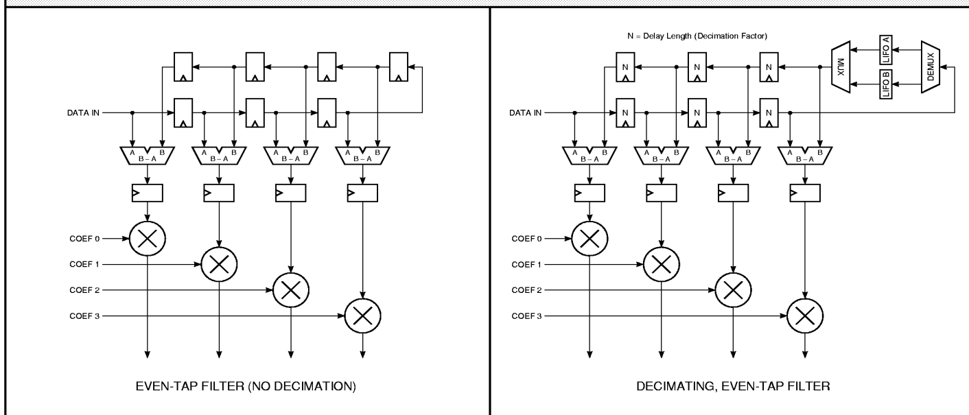
FIGURE 6. ODD-SYMMETRIC COEFFICIENT FILTER CONFIGURATIONS
