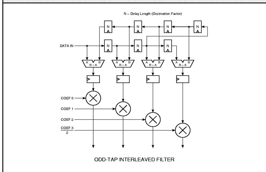
FIGURE 7. INTERLEAVED COEFFICIENT FILTER CONFIGURATION
