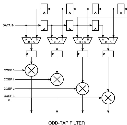
ODD-TAP FILTER
