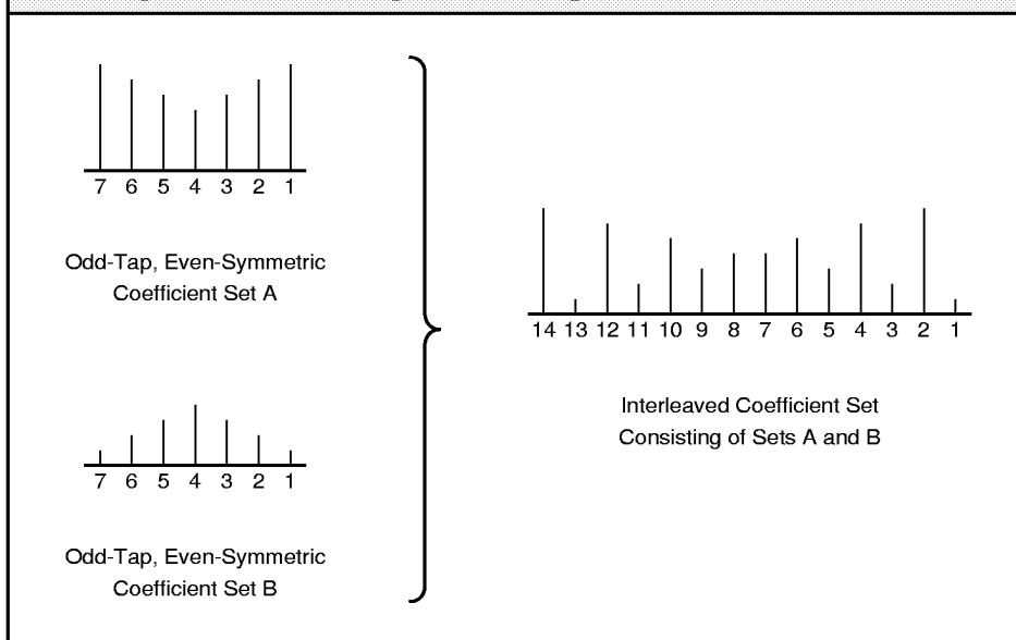
FIGURE 8. INTERLEAVED COEFFICIENT SET EXAMPLE
