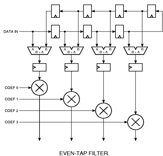
EVEN-TAP FILTER
