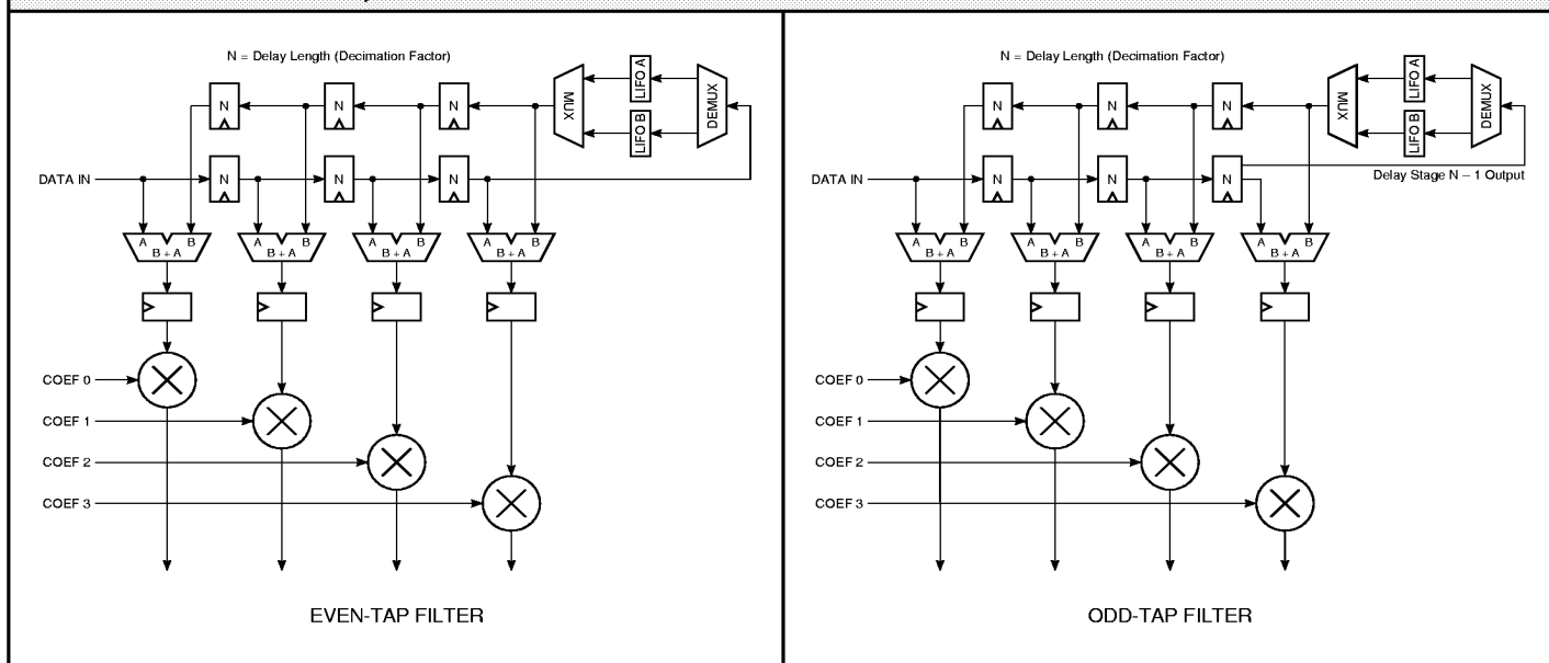
FIGURE 5. DECIMATING, EVEN-SYMMETRIC COEFFICIENT FILTER CONFIGURATIONS
