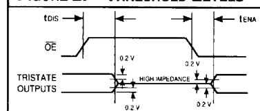
FIGURE 2. THRESHOLD LEVELS
