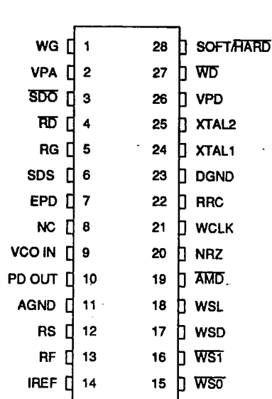
28-pin DIP
