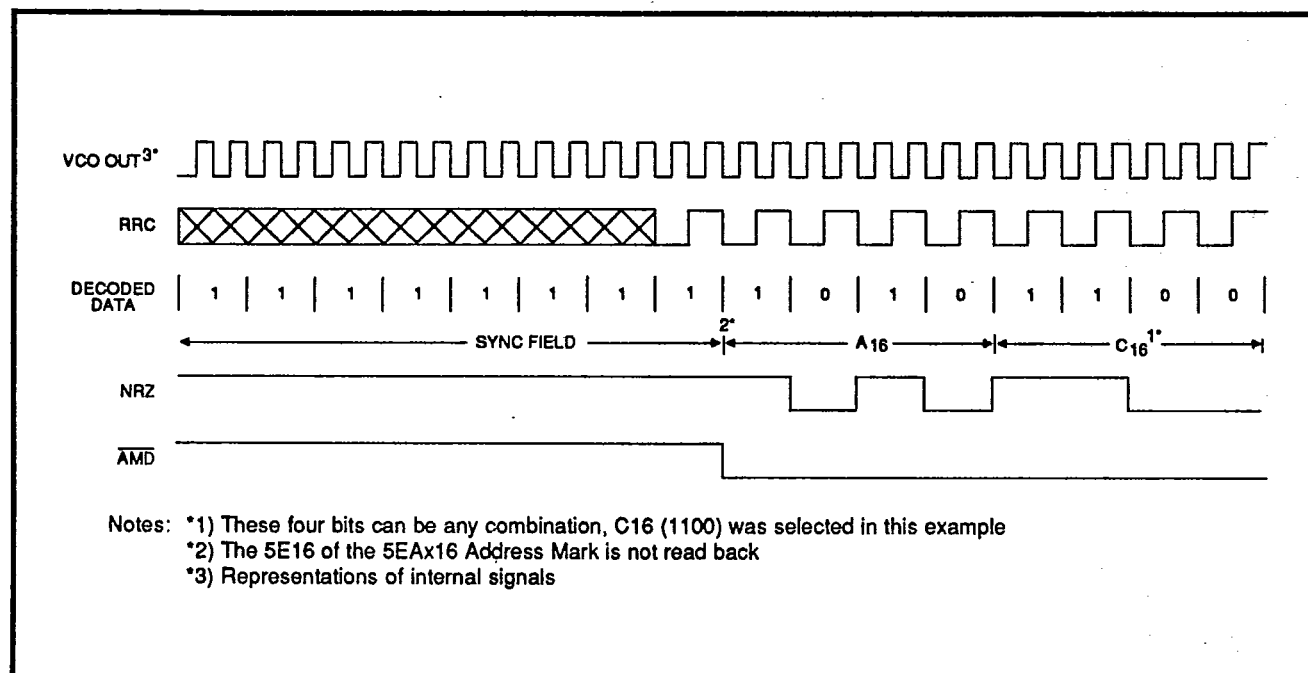
FIGURE 5: Address Mark Detection and NRZ Output Waveform
