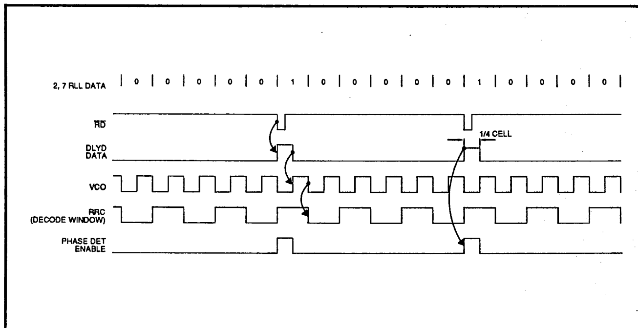
FIGURE 2: Data Synchronization Waveform Diagram
