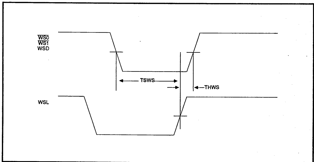
FIGURE 11: Control Timing
