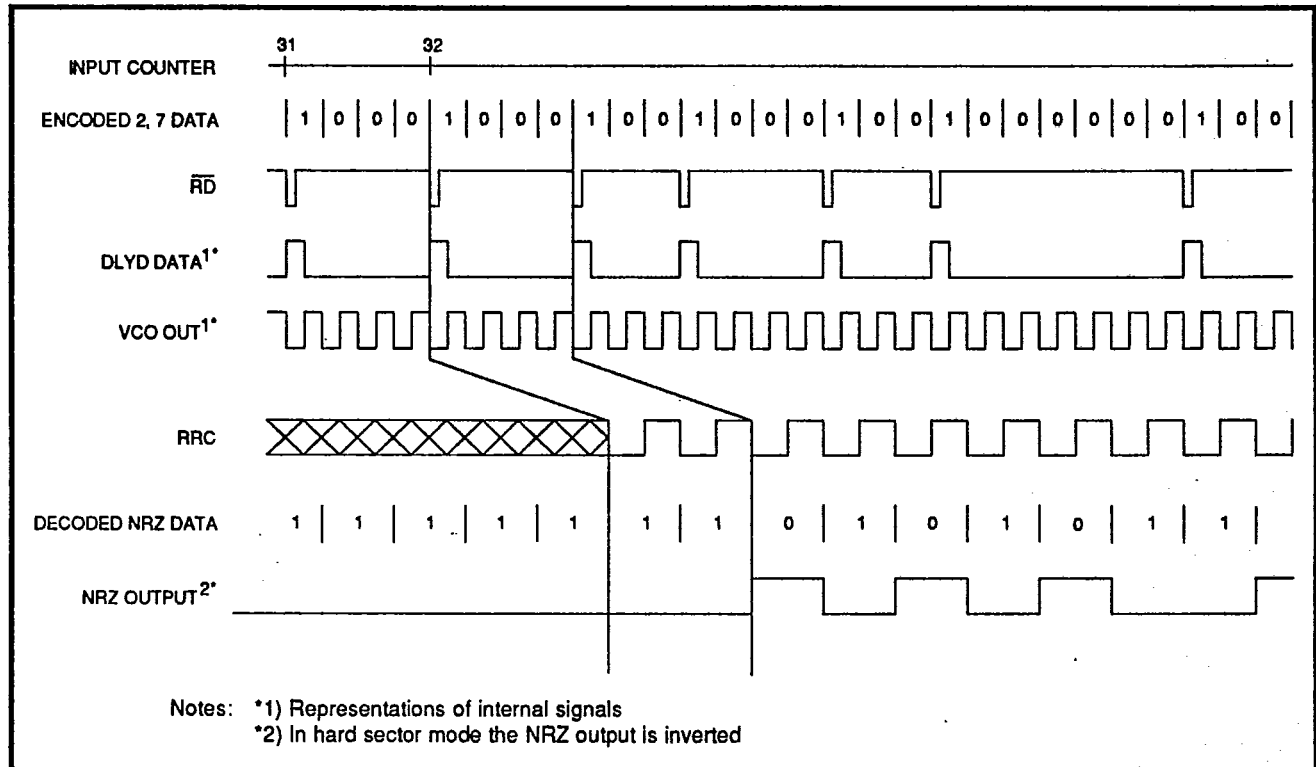
FIGURE 7: Hard Sector Mode Decode Timing
