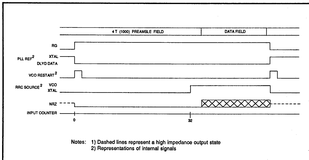
FIGURE 6: Hard Sector Mode Timing Diagram
