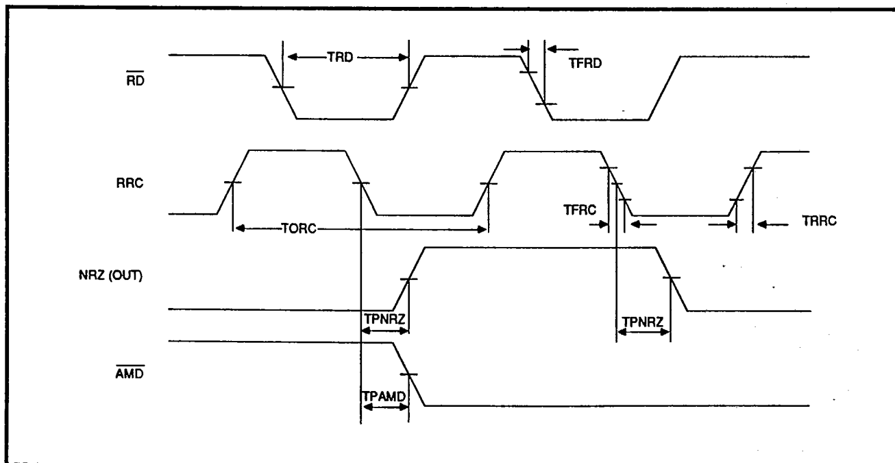
FIGURE 9: Read Timing
