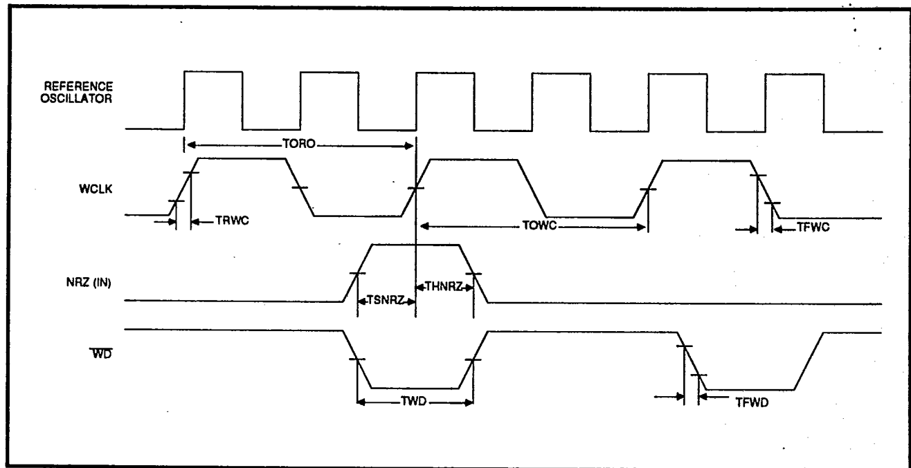
FIGURE 10: Write Timing
