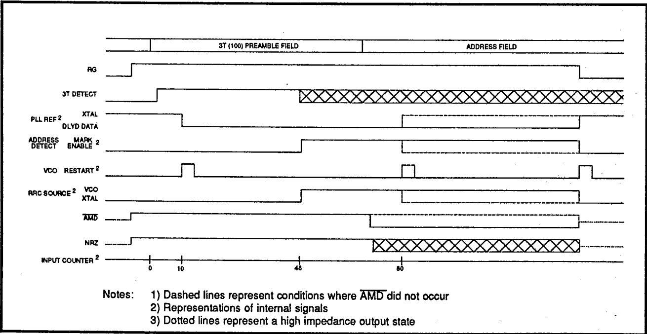
FIGURE 4: Soft Sector Mode Timing Diagram
