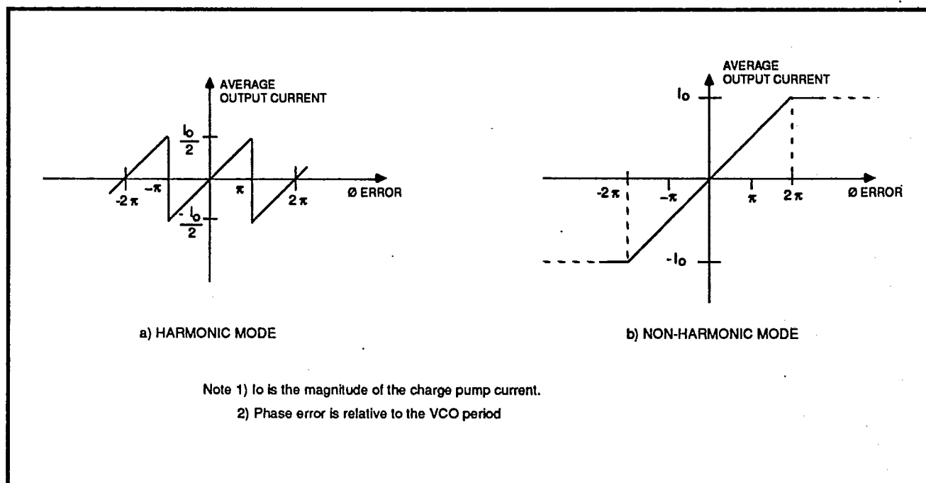
FIGURE 1: Phase Detector Transfer Function
