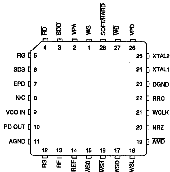
28-pin PLCC
