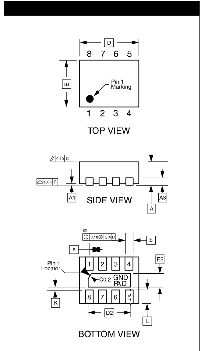
Dimensions for 8-Lead, 0.4mm pitch μDFN package
