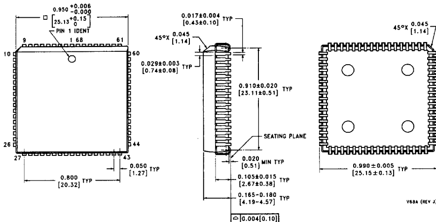
68-Pin Plastic Leaded Chip Carrier (V) Order Number NSAM266SCA/V NS Package Number V68A
