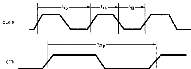
FIGURE 1-22. CTTL and CLKIN Timing
