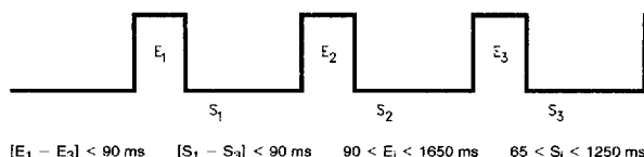
FIGURE 2-2. Busy-Tone Detector—Cadence Specification
