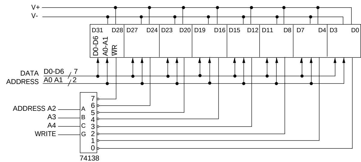
Figure 3. Typical interconnection for 32 characters
