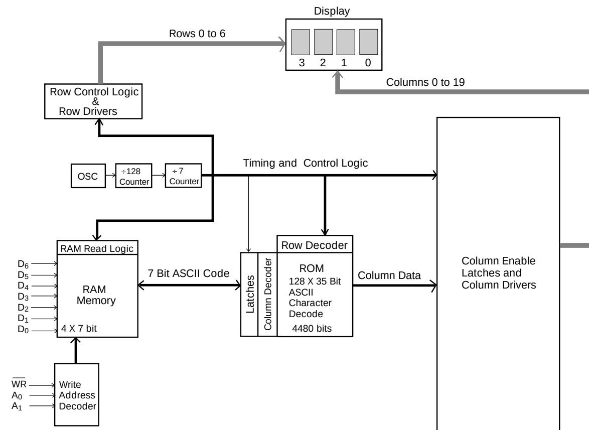
Figure 4. Block diagram
