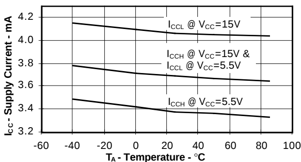
Figure 7. Typical supply current vs. temperature
