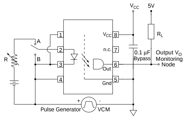
Figure 31. Test circuit for common mode transient immunity and typical waveforms—SFH6705 L
