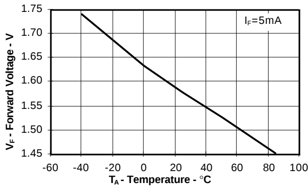
Figure 4. Typical forward input voltage vs. temperature
