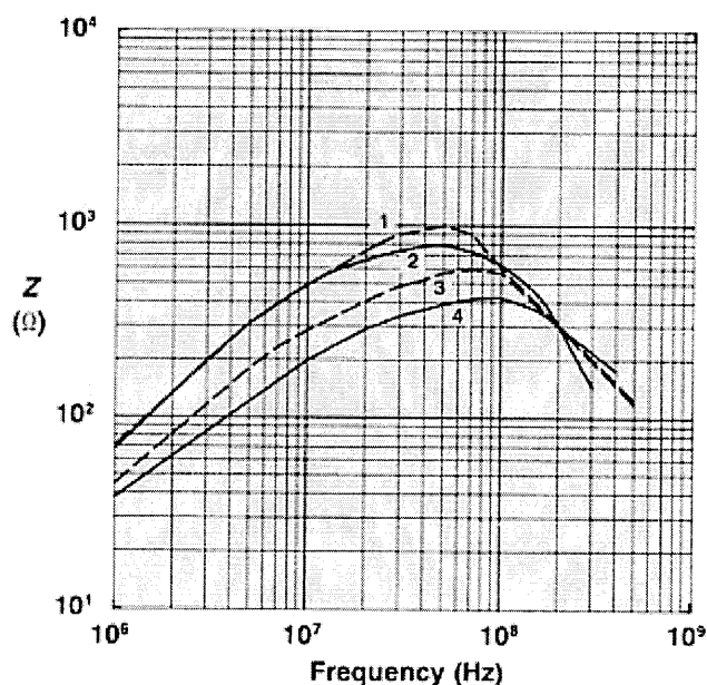
Figure 47 Impedance vs. Frequency for wound six hole beads in 43 material.
