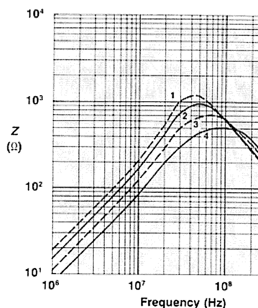
Figure 48 Impedance vs. Frequency for wound six hole beads in 61 material.
