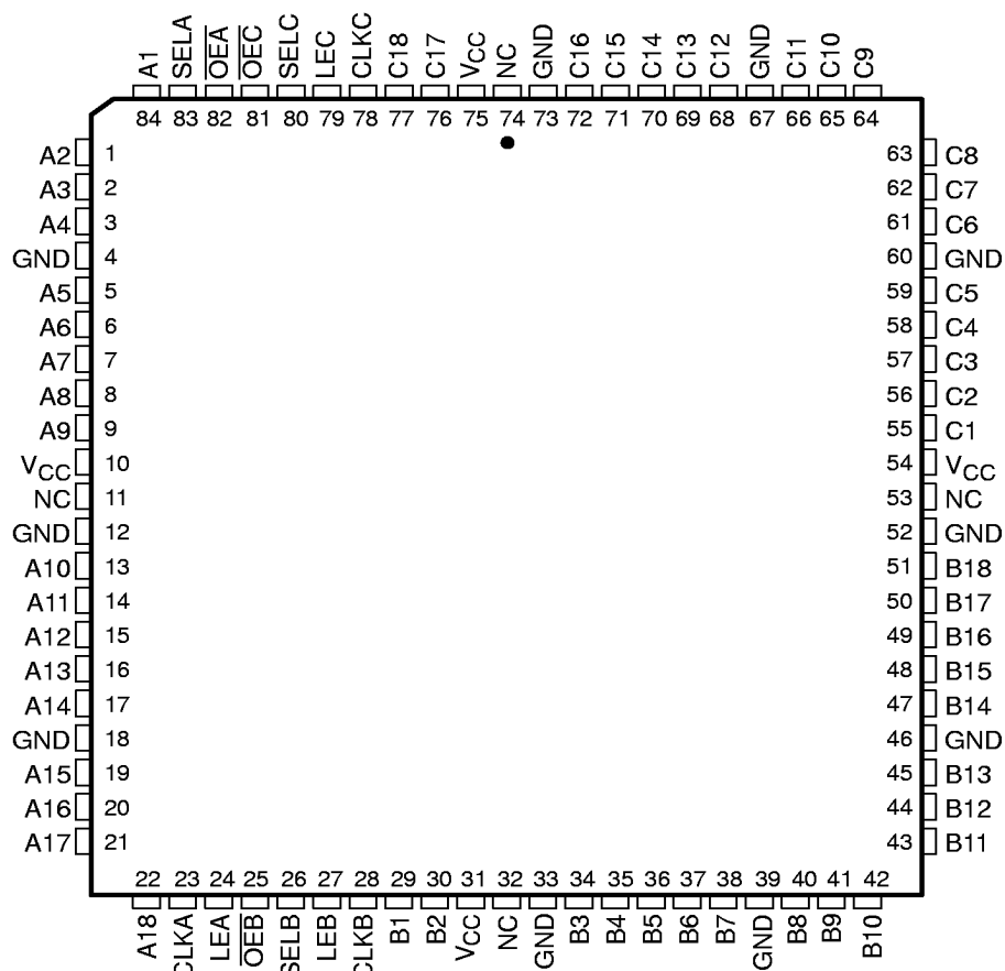
SN54ABTH32318 . . . HT PACKAGE (TOP VIEW)
