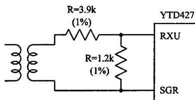
Figure 4.1: Receive Interface Connection
