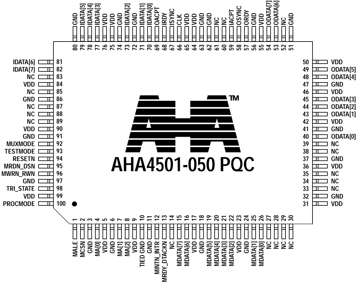
Figure 15: Pinout – 100 MQFP
