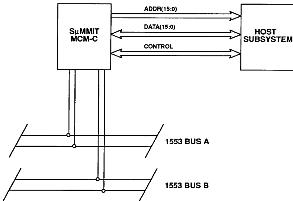
Figure 16a. SμMMIT MCM-C General System Diagram
