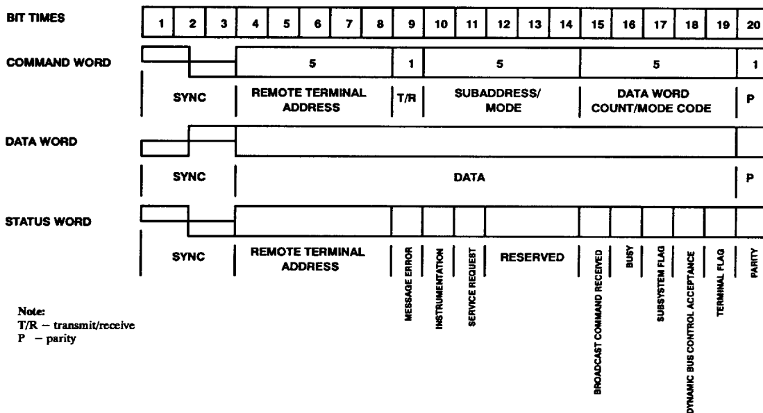
Figure 19. MIL-STD-1553B Word Formats
