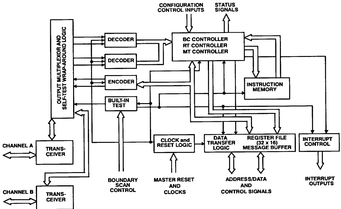
Figure 1. UT69151 LX & DX S \mu MMIT MCM-C Block Diagram
