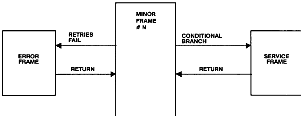
Figure 7a. Minor Frame Branching
