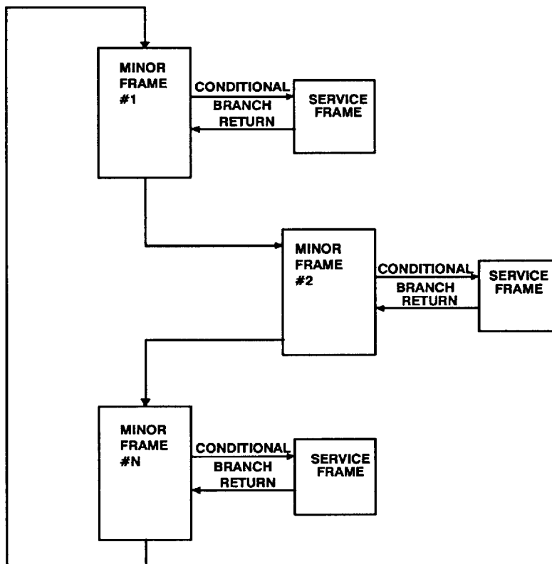
Figure 7b. Major Frame Sequencing
