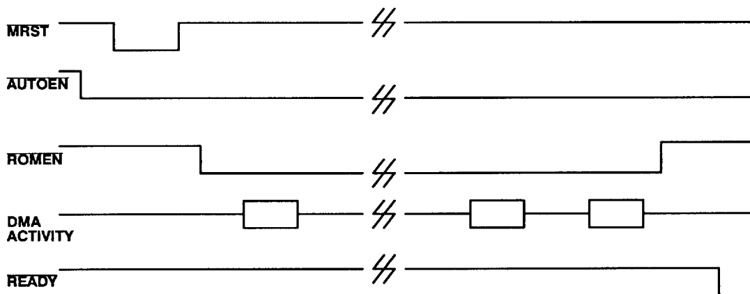
Figure 14b. Auto-Initialization DMA Sequence
