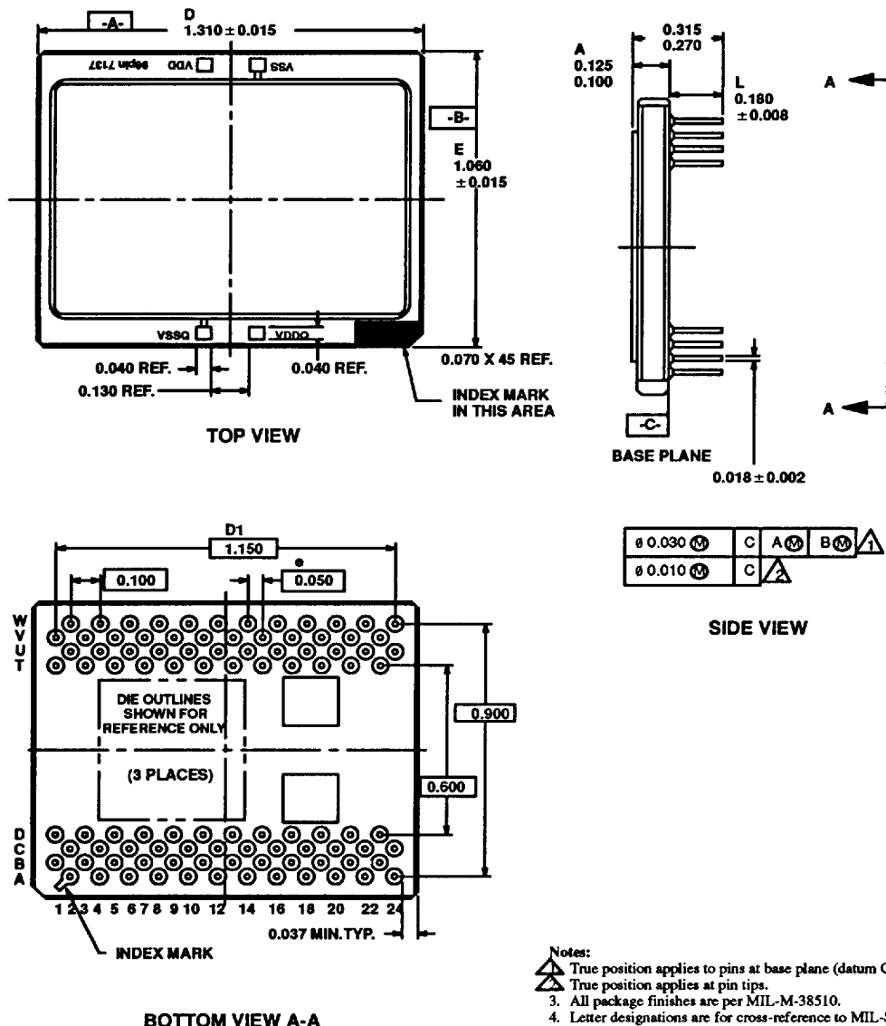
Figure 30. 96-Pin Pingrid Array
