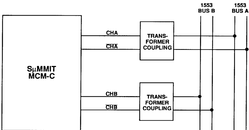
Figure 16b. SμMMIT to MIL-STD-1553 Interface Diagram
