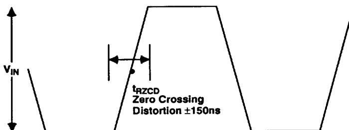
Figure 29. Receiver Input Zero Crossing Distortion ( t_{RZCD} )
