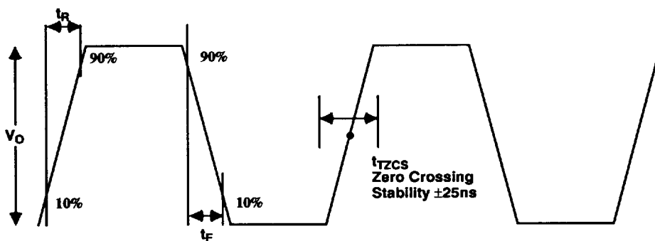
Figure 28. Transmitter Output Zero Crossing Stability ( t_{ZCS} , t_R , t_F )
