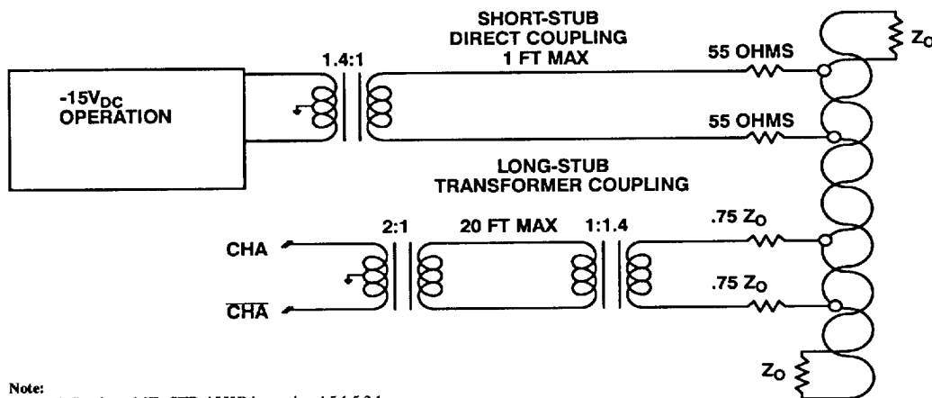
Figure 17a. LX-15 Bus Coupling Configuration
