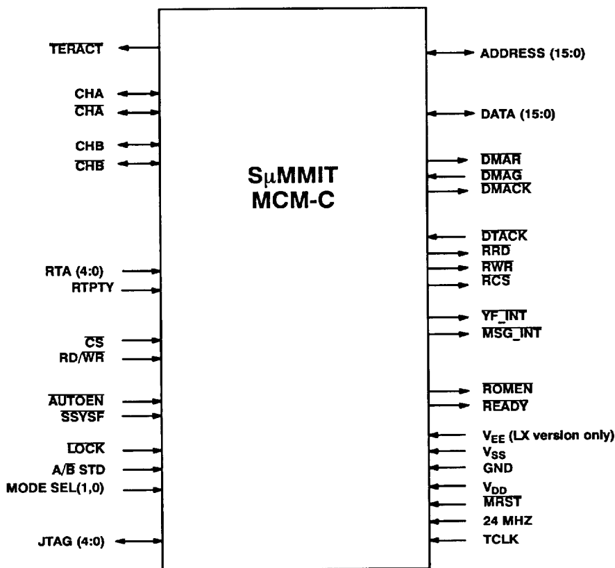
Figure 18. SμMMIT MCM-C Functional Pin Description
