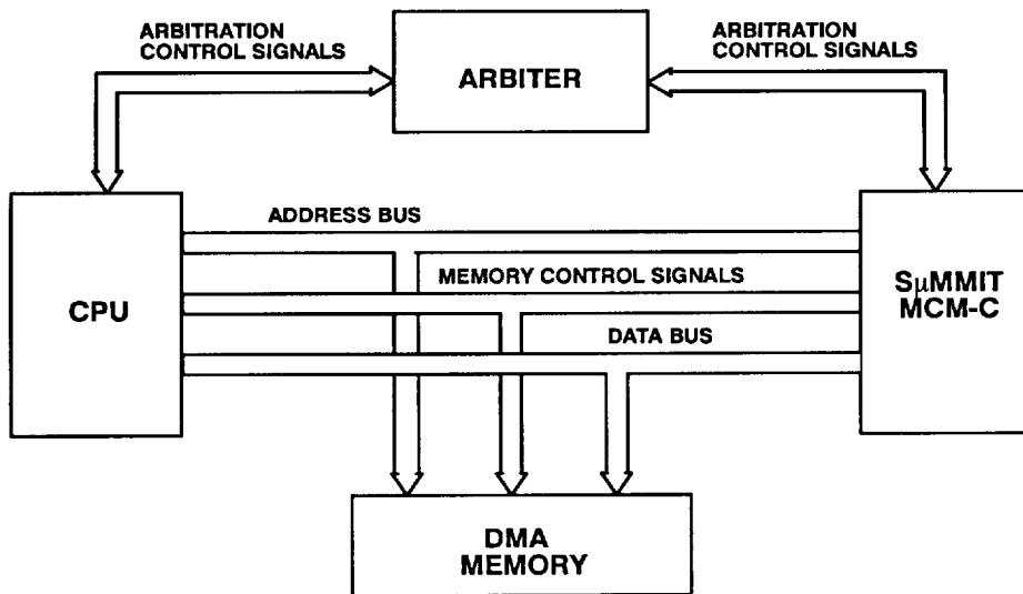
Figure 15a. DMA System Configuration
