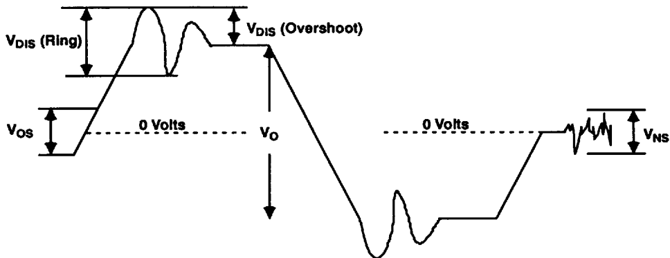
Figure 27. Transmitter Output Characteristics ( V_{DIS} , V_{OS} , V_{NS} , V_O )
