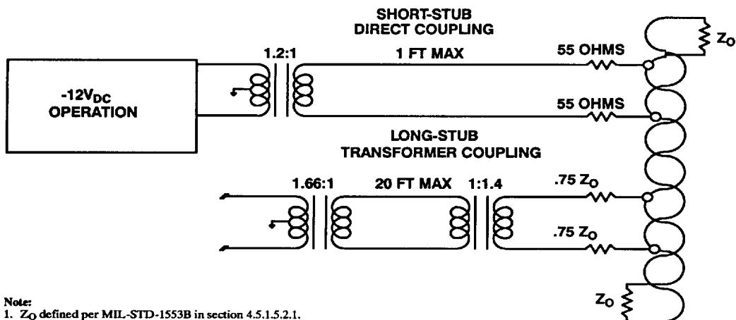
Figure 17b. LX-12 Bus Coupling Configuration
