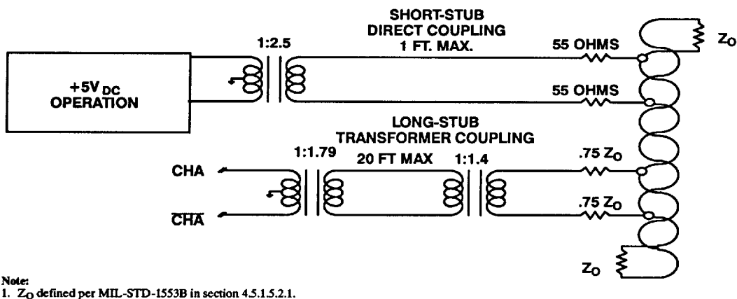
Figure 17c. DX Bus Coupling Configuration
