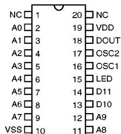
HT6012 – 20 SOP
