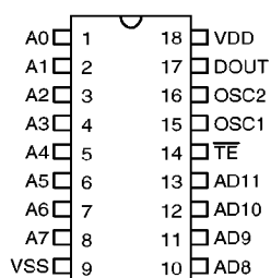
HT6010 – 18 DIP
