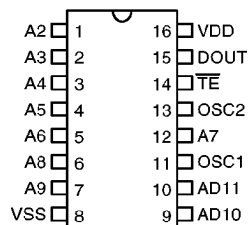
HT6013 – 16 DIP/SOP/NSOP
