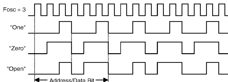
Address/Data bit waveform
