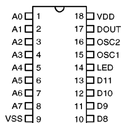
HT6014 – 18 DIP
