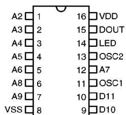
HT6015 – 16 DIP/SOP/NSOP
