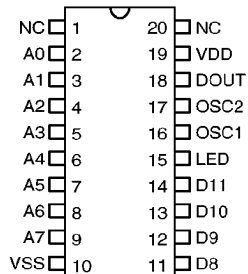
HT6014 – 20 SOP
