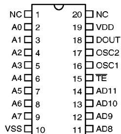
HT6010 – 20 DIP/SOP
