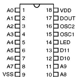
HT6012 – 18 DIP
