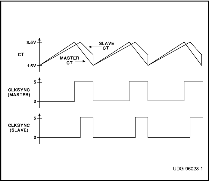
Figure 3. Oscillator waveforms.
