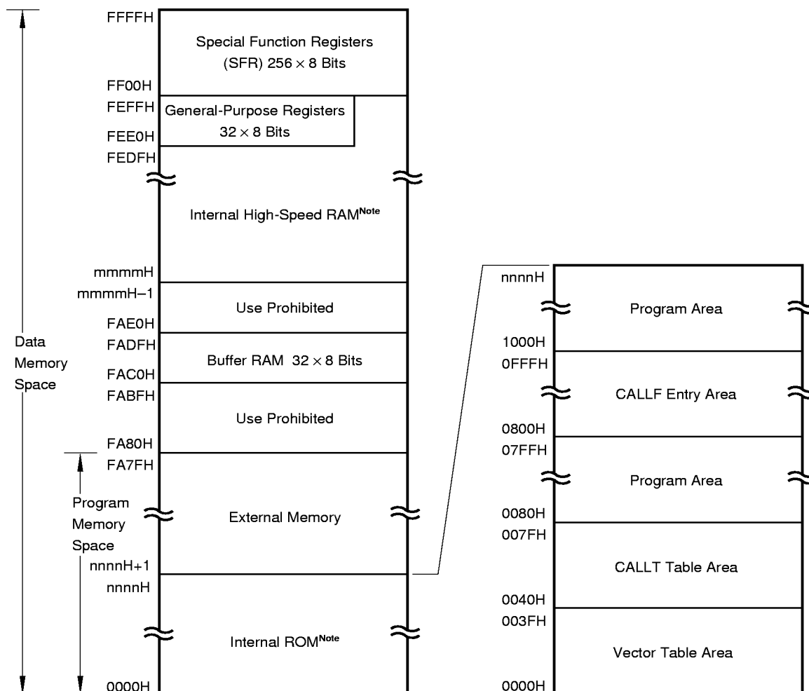
Figure 4-1. Memory Map
