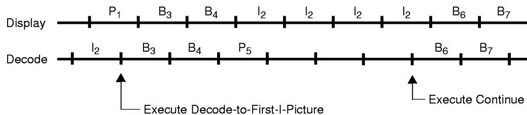
Figure 32. Decode-to-First-I-Picture
