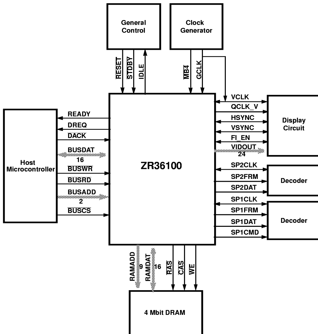
Figure 3. Generic ZR36100 Schematic Diagram
