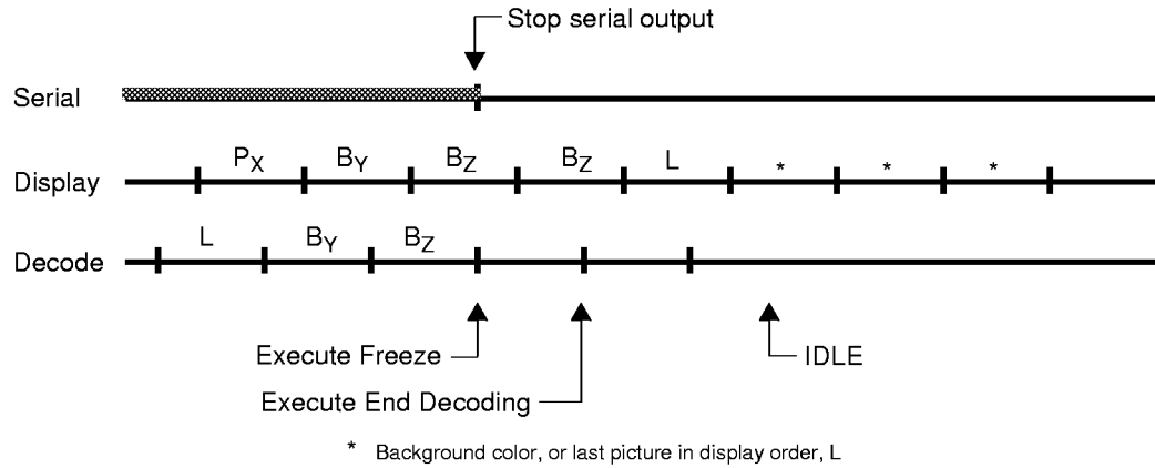
Figure 30. End Decoding
