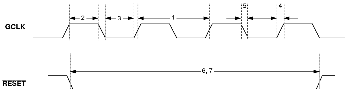
Figure 33. GCLK and RESET timing
