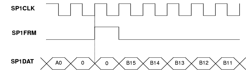
Figure 25. Beginning of serial port frame with pulse frame sync signal, length of previous frame is 18 clocks
