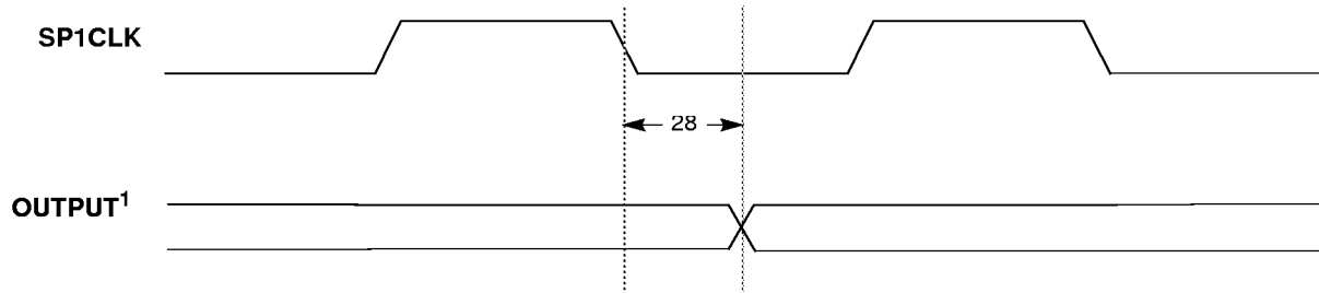
Figure 39. Serial Port 1 timing (SP1FRM transition mode)
