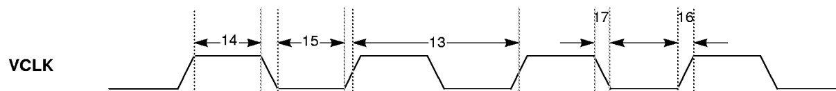
Figure 34. VCLK timing
