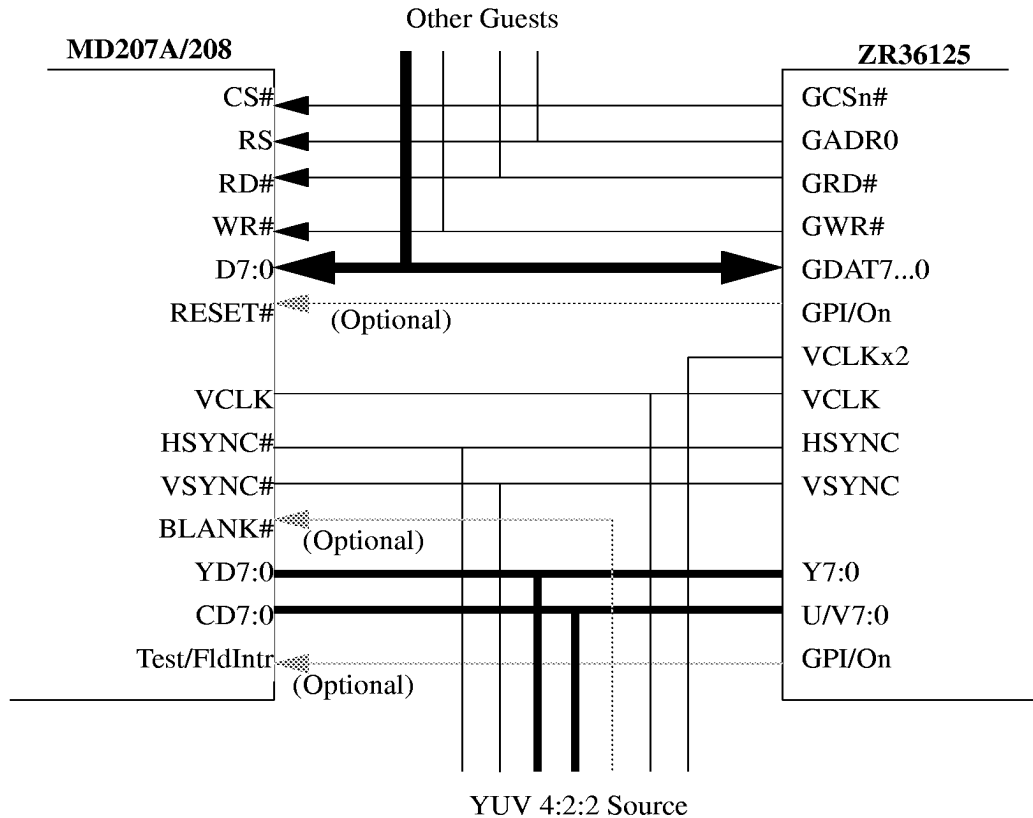
Figure 9: ZR36125 - MD207A/208 Basic Interconnection
