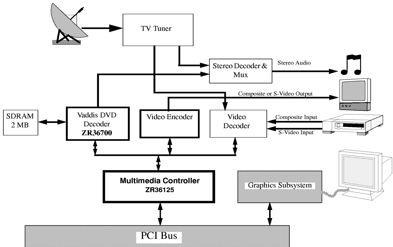
Figure 1: Block Diagram of A DVD/TV Subsystem for PCI Computers
