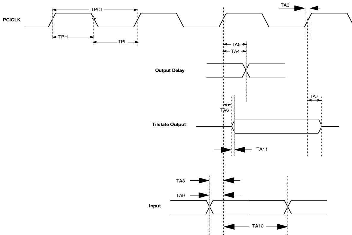
Figure 4: PCI Bus Interface Timing
