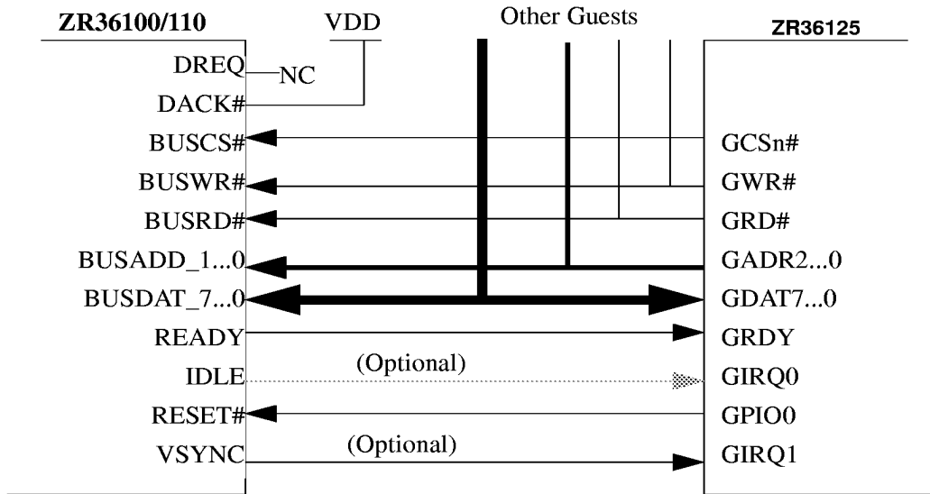
Figure 8: ZR36125 - ZR36100/ZR36110 Host (Guest) Bus Interconnection
