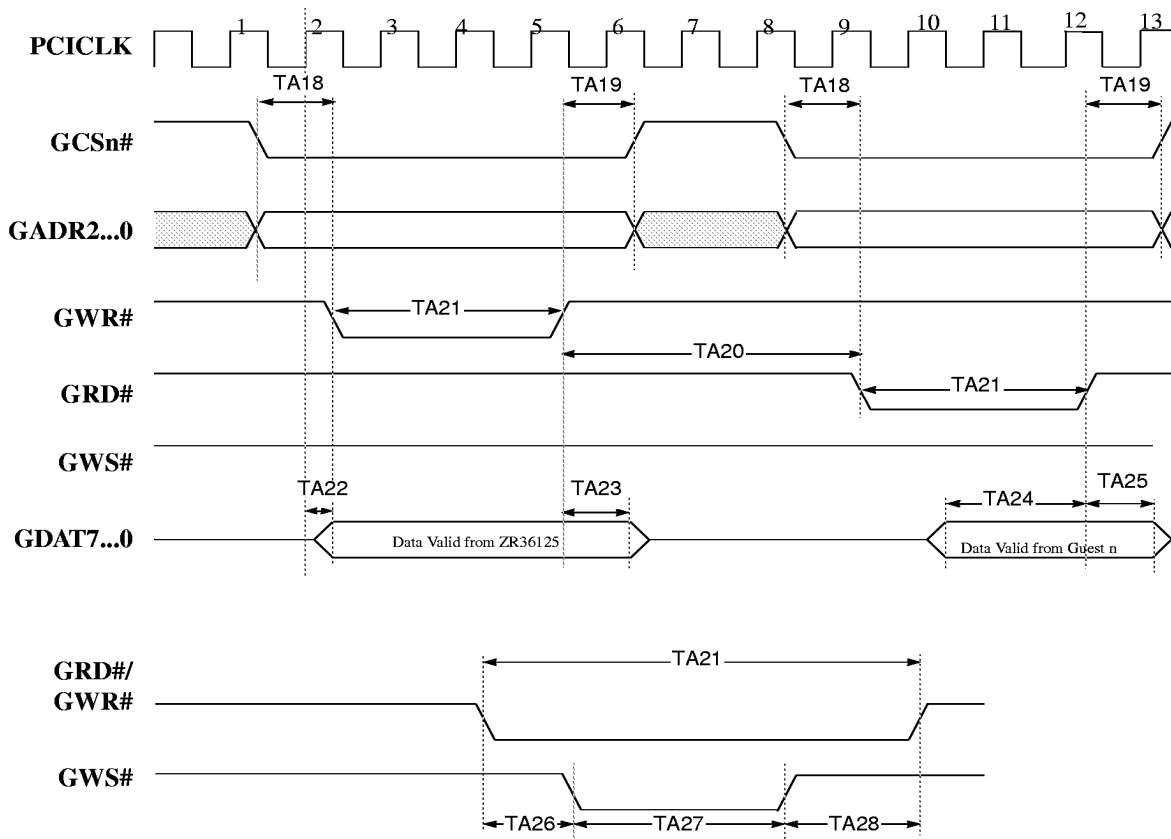
Figure 6: GuestBus Timing
