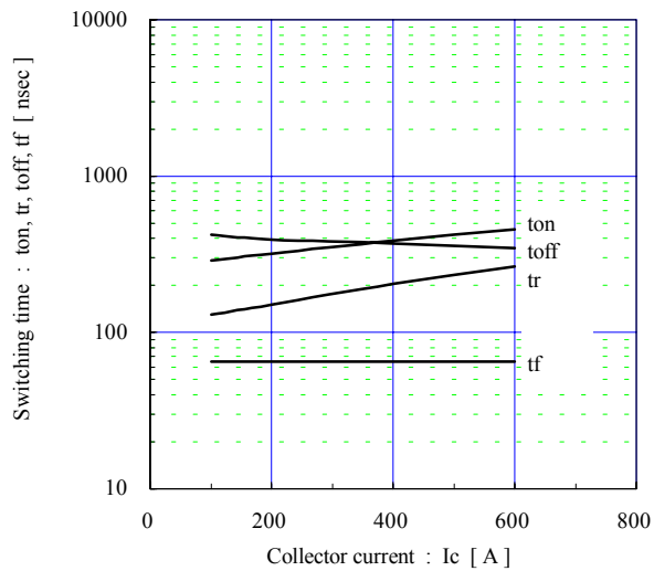
Switching time vs. Collector current (typ.) V_{cc}=600V , V_{GE}=\pm 15V , R_g=1.5\Omega , T_j=25^\circ C
