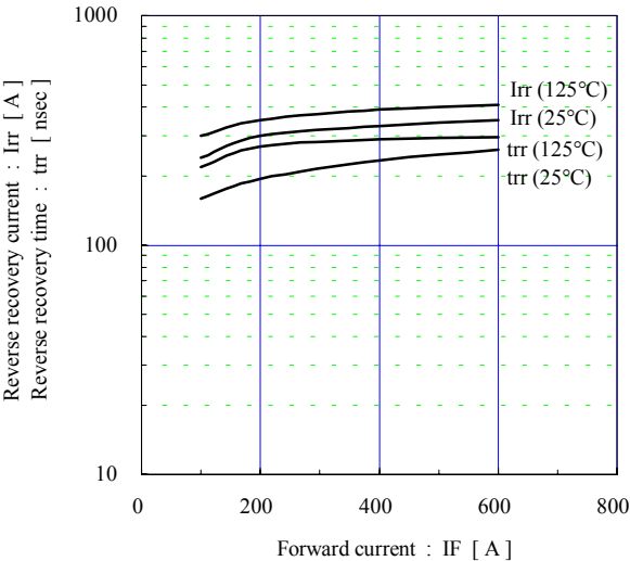
Reverse recovery characteristics (typ.) Vcc=600V, VGE=±15V, Rg=1.5Ω
