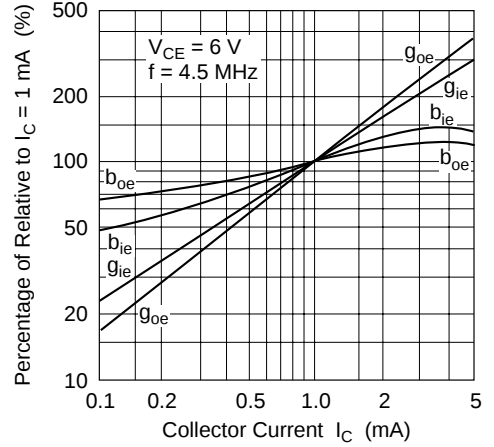
Input/Output Admittance vs. Collector Current
