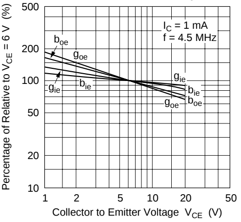
Input/Output Admittance vs. Collector to Emitter Voltage
