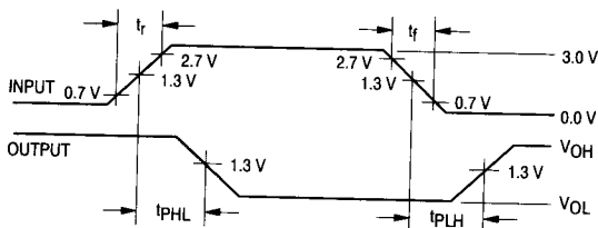
WAVEFORMS
