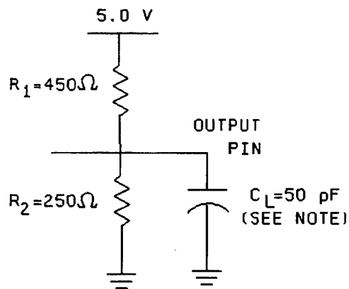
CIRCUIT B OR EQUIVALENT
