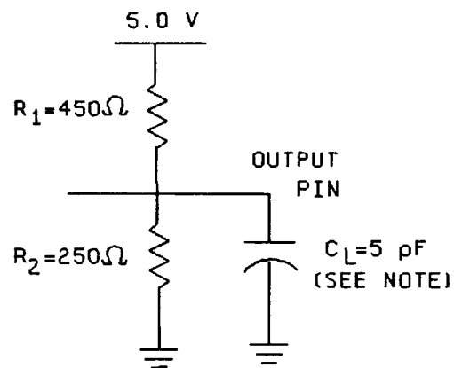
CIRCUIT A OR EQUIVALENT
