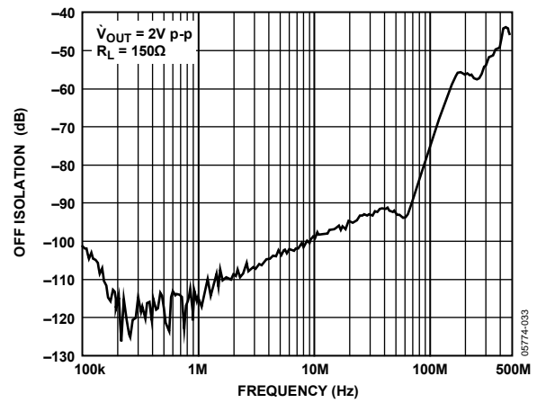
Figure 32. AD8107 Off Isolation, Input/Output
