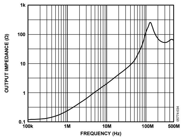
Figure 33. AD8107 Output Impedance, Enabled
