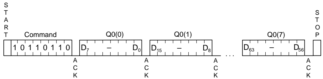
Figure 11. Initialize Authentication
