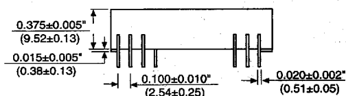
SIDE VIEWS
