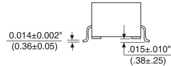
END VIEWS
