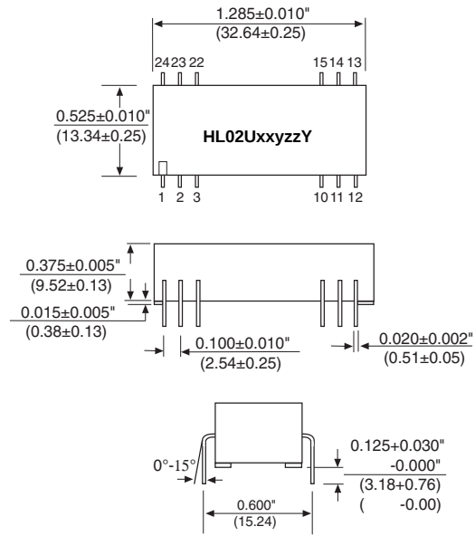
SIDE VIEWS
