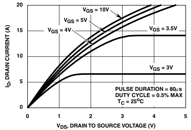
FIGURE 8. SATURATION CHARACTERISTICS
