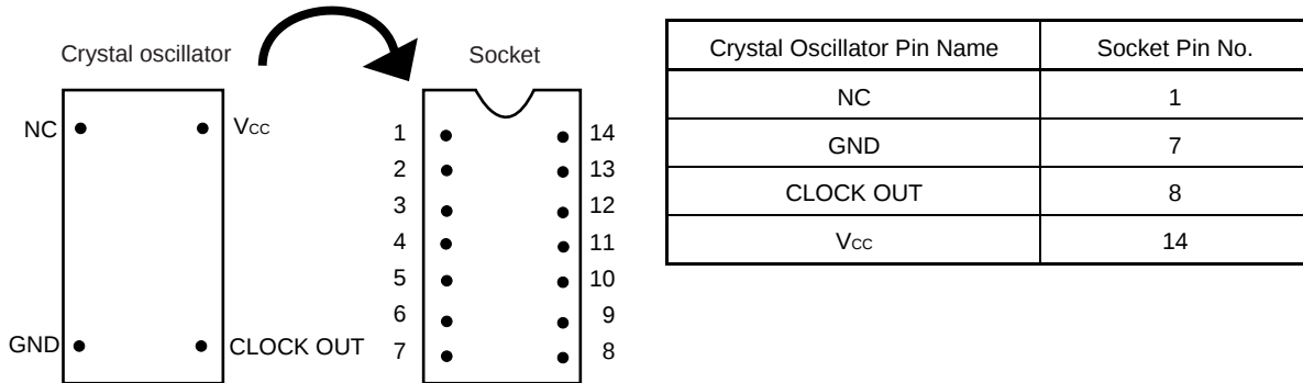
Figure 3-12. Pin Alignment of Crystal Oscillator and Socket
