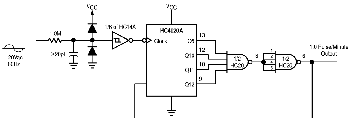
Figure 7. Time-Base Generator
