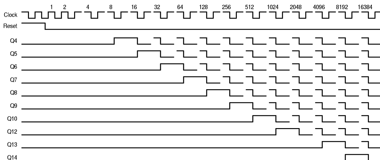
Figure 6. Timing Diagram
