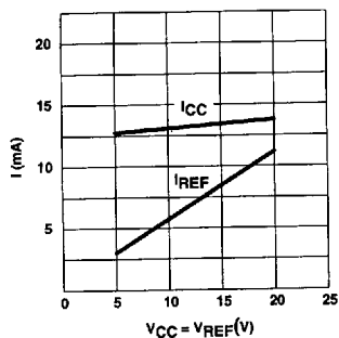
Figure 3. I_{REF} and I_{CC} vs Voltage ( T_{amb} = +25^{\circ}C )
