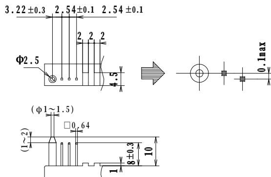
Details of control terminals
