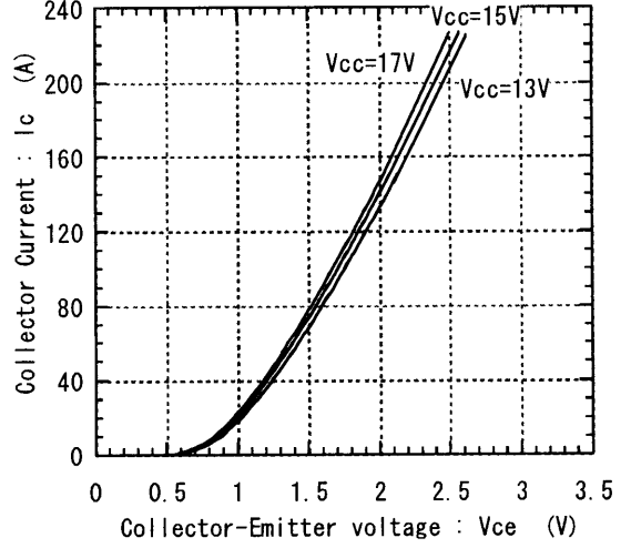
Collector current vs. Collector-Emitter voltage Tj=25°C (Terminal)
