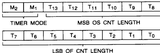
Figure 5. Timer Format
