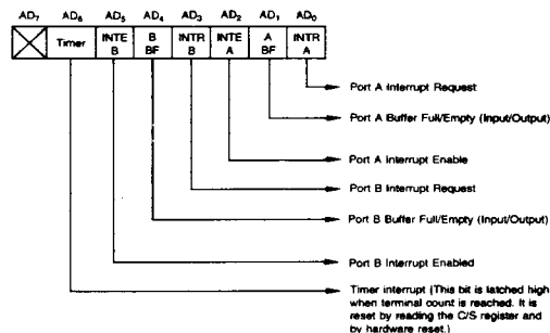
Figure 3. Command/Status Register Status Word Format
