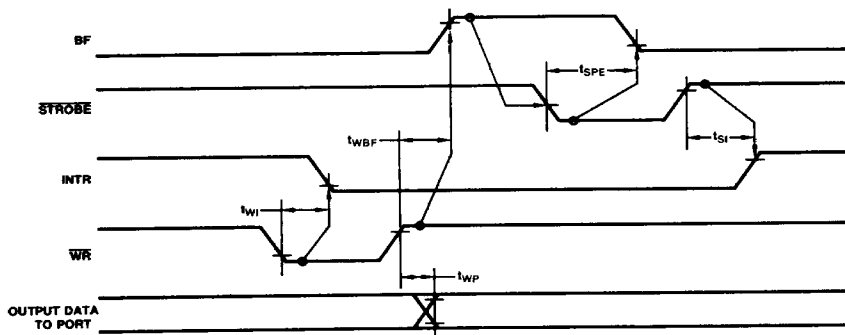
Strobed Output Mode
