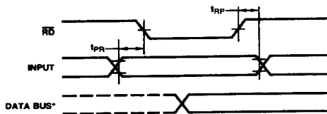
Basic I/O Timing Waveform
