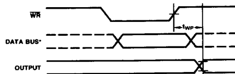
Basic I/O Timing Waveform
