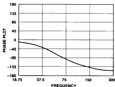
Figure 4. AD2S46 Phase Plot
