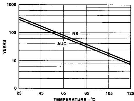
Figure 5. AD2S46 MTBF vs. Temperature
