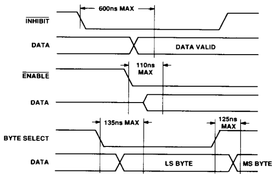
Figure 2. Timing Diagrams
