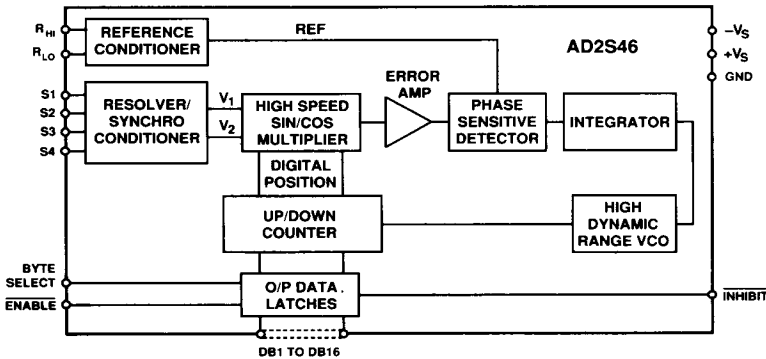
AD2S46 Functional Block Diagram
