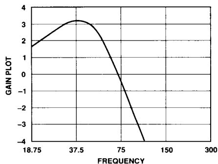
Figure 3. AD2S46 Gain Plot
