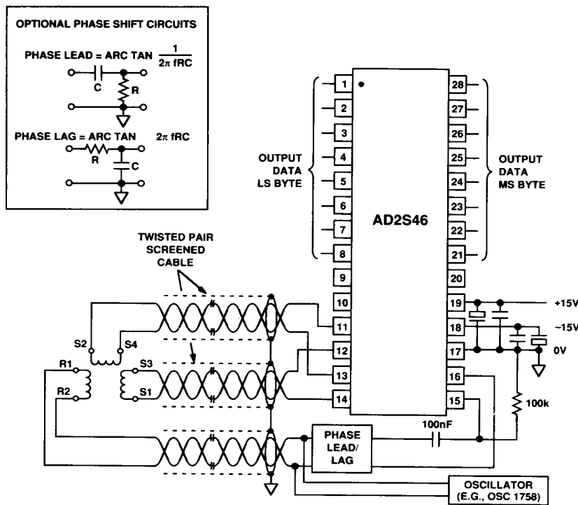
Figure 1. Connection Diagram
