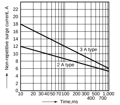
2-(2). Non-repetitive surge current vs. carrying time (DC output type)
