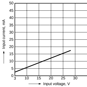
3. Input voltage vs. input current
