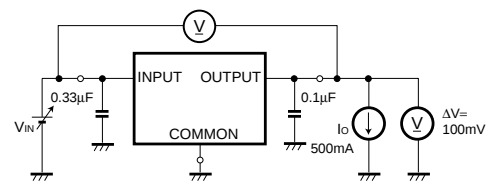
Fig. 4 Measurement circuit for Minimum I/O voltage differential
