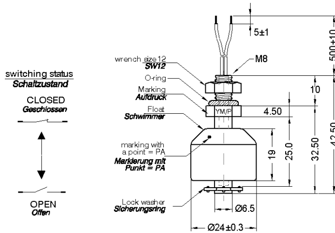
Abmessungen / dimensions (mm) Tolerances acc. to DIN ISO 2768-m
